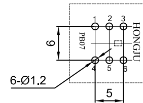
PCB HOLE( BOTTON VIEW)
